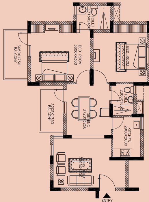
ASTER\ COUR 2BHK TYPE-C TOWER= 2
