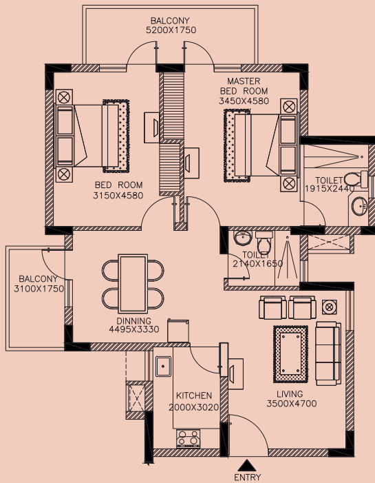
ASTER\ COUR 2BHK TYPE-B TOWER= 2
